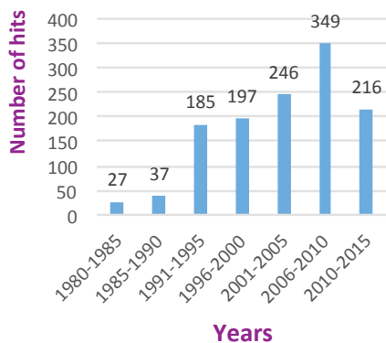
FIGURE 1. Search statistic of articles published in Geochimica et Cosmochimica Acta that used the key word “kinetics.” Data are arranged in five year intervals. Search was made in August 2015. (Color online.)
